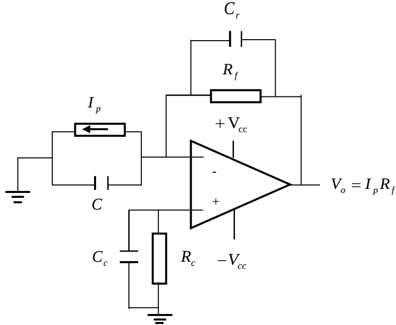
Figure 3. Transimpedance amplifier circuitry.
