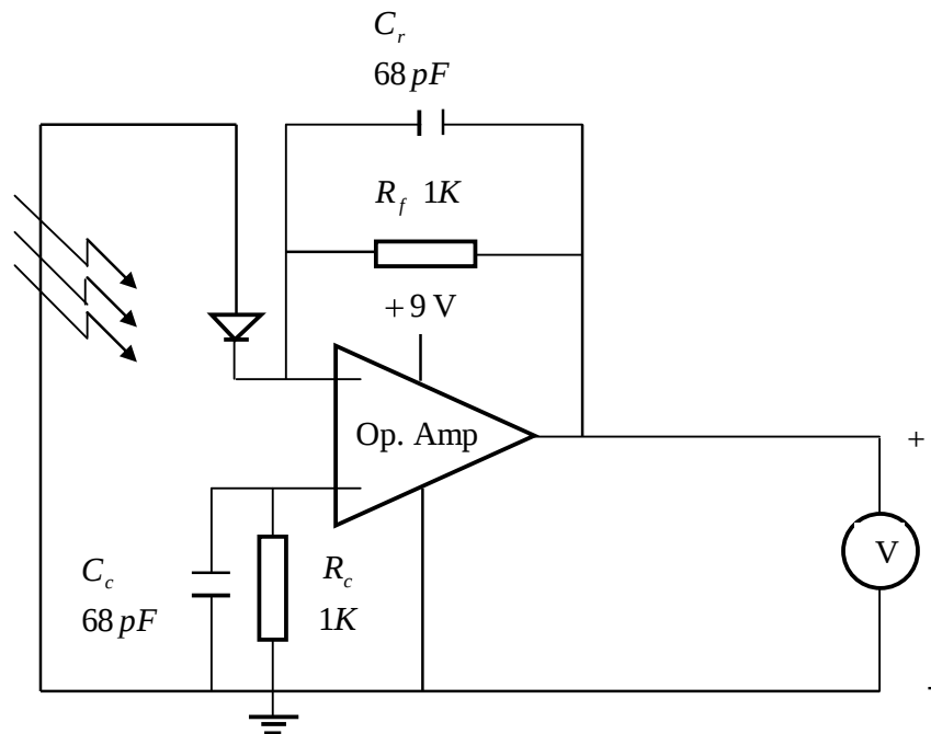
Figure 2. Pyranometer circuit diagram.
