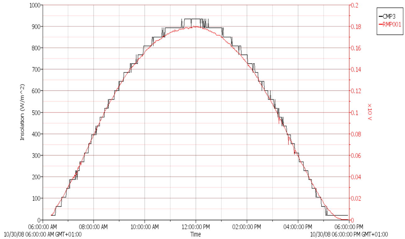
Figure 4. Graph of solar radiation measured with CMP3 and RMP001 versus time on 30 th October, 2008.
